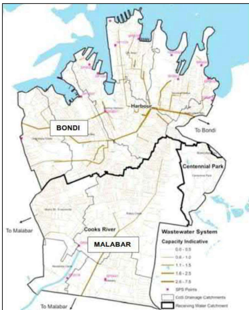
Figure 8: Sydney Water Sewer Catchment Plan (Sydney Water, 2015)
