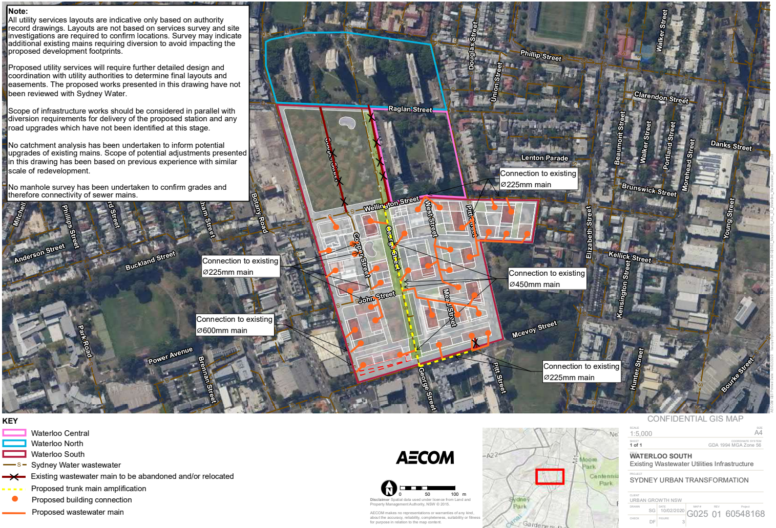
Figure 9: Proposed Waterloo Wastewater Plan
